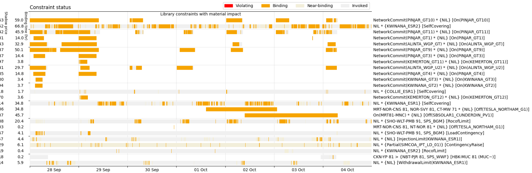
Figure 3 – Binding summary of library constraints.
