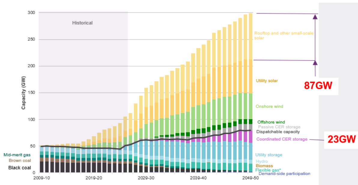
Figure 5 – Step Change Scenario – GW Generator and Storage Capacity Plan
