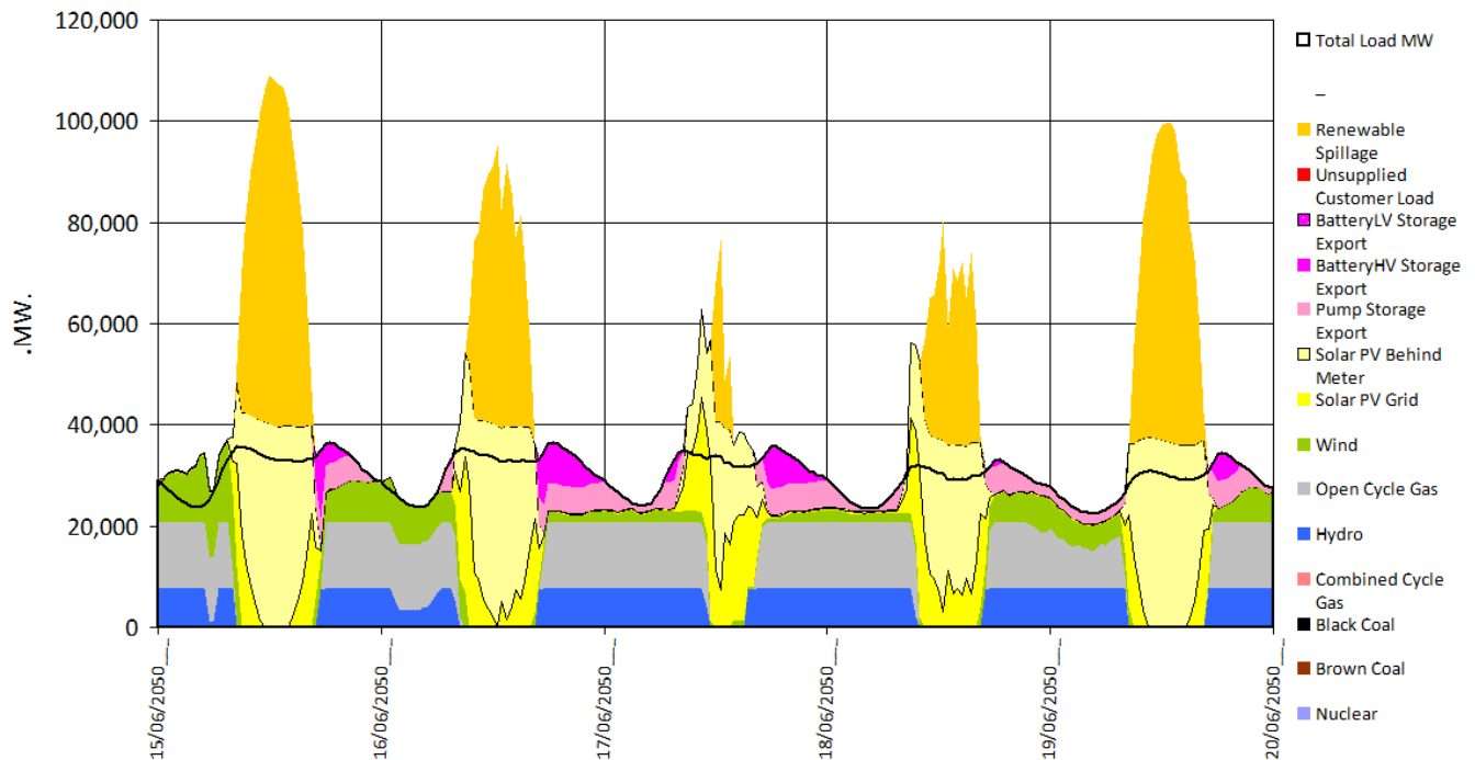
Figure 3 – Step Change Scenario – EPC Model of June 2050 - EPC Model Generation and Storage Resource with the 2050 Load Reduced to 297 TWh
