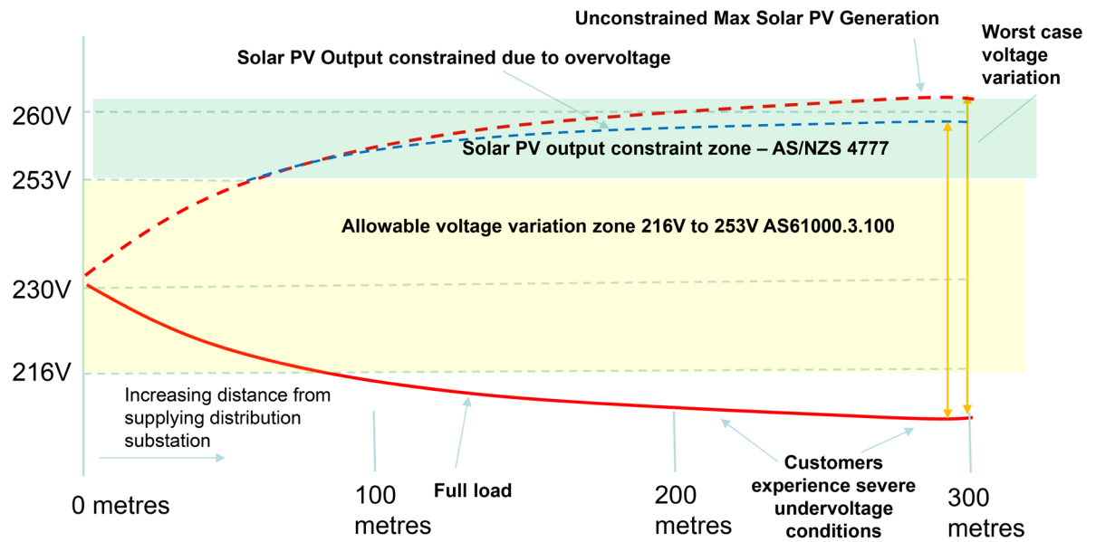
Figure A4.5 -LV Feeder Voltage Profile with Solar PV and Reduced Distribution Supply Voltage
