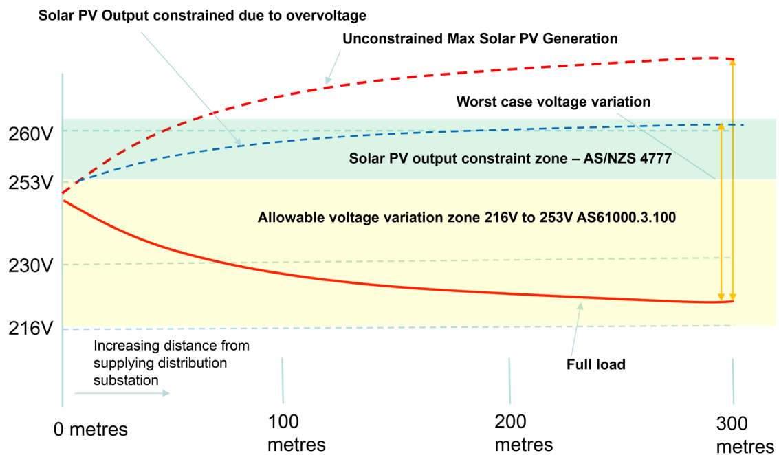
Figure A4.4 - LV Feeder Voltage Profile with Solar PV
