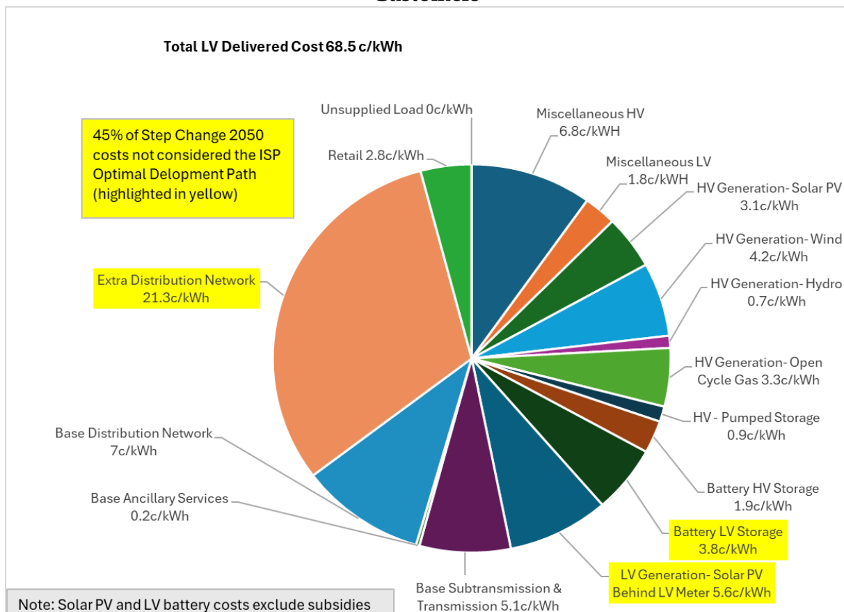
Figure 4 – 285 TWh Step Change Scenario– EPC Model of Delivered Cost to LV Customers
