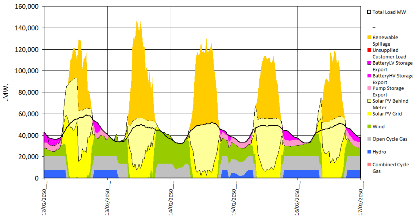
Figure 1 – Step Change Scenario – EPC Model Summer Projected 2050 Generation Profile
