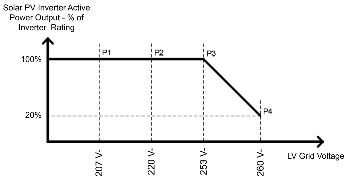
Figure A4.2 - Solar PV Inverter – Typical Setting/Characteristics
